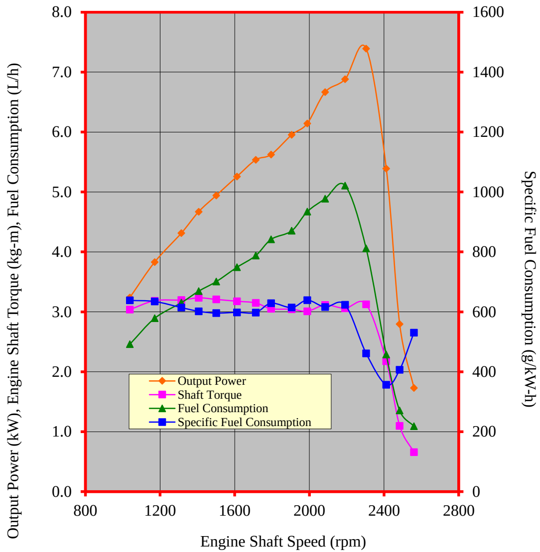
Figure 3. Performance characteristic curves of the EMEI EMZ185N diesel engine
