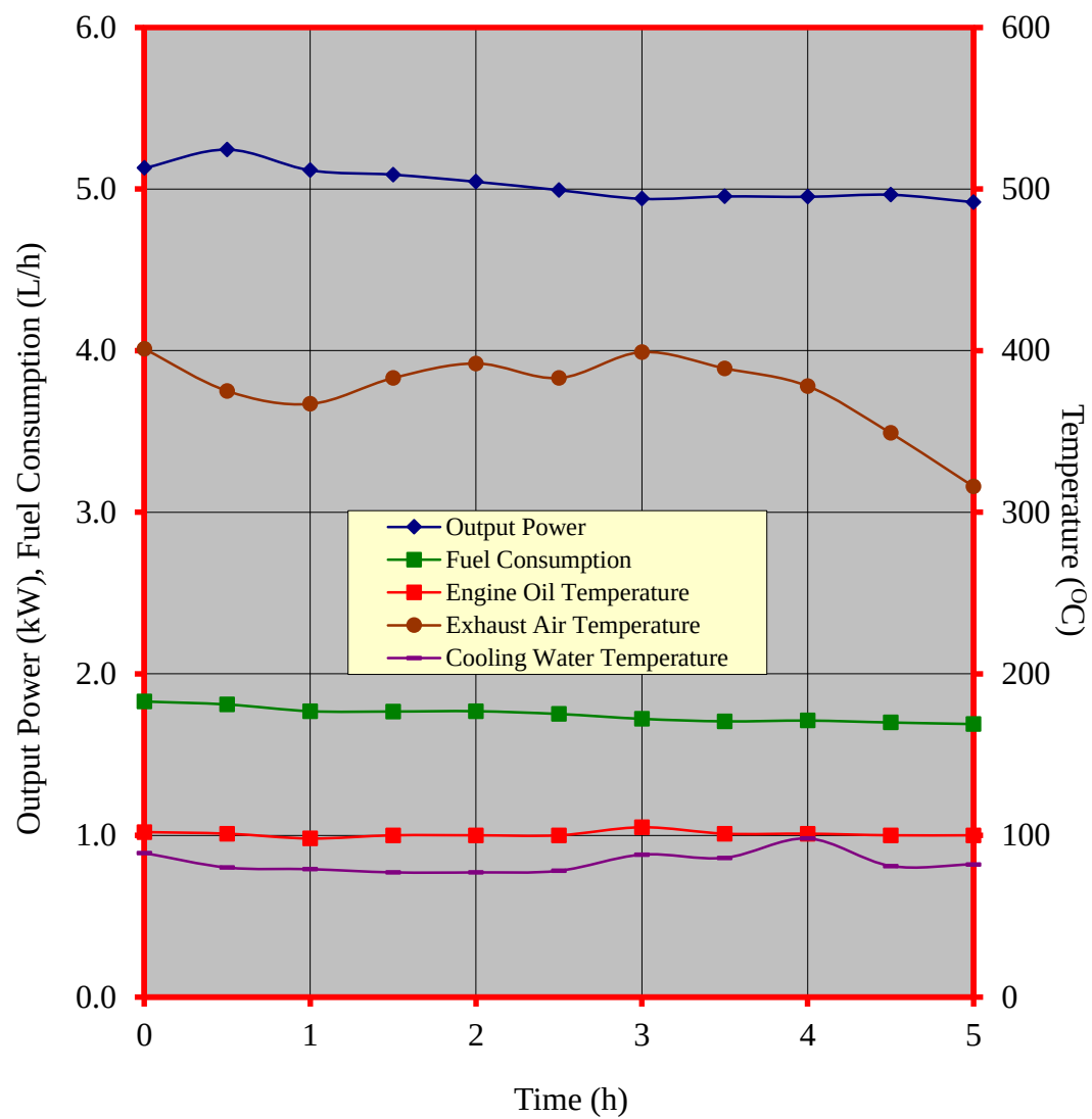
Figure 4. Performance characteristic curves during the continuous running test of the EMEI EMZ 185N diesel engine
